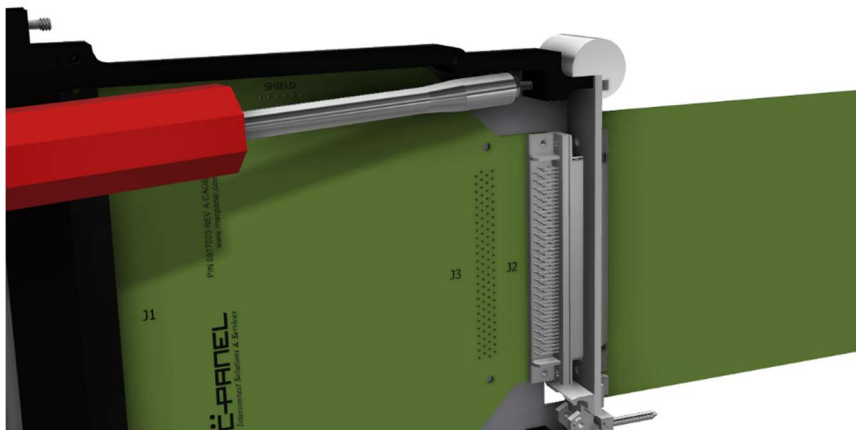
Figure 14 Tighten the T bolt ensuring correct alignment.
