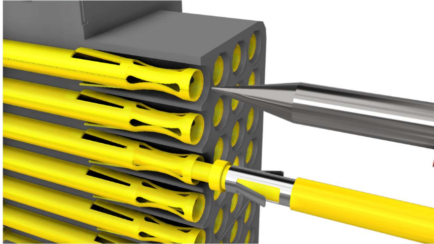
Figure 21 1mm contact inserted.
