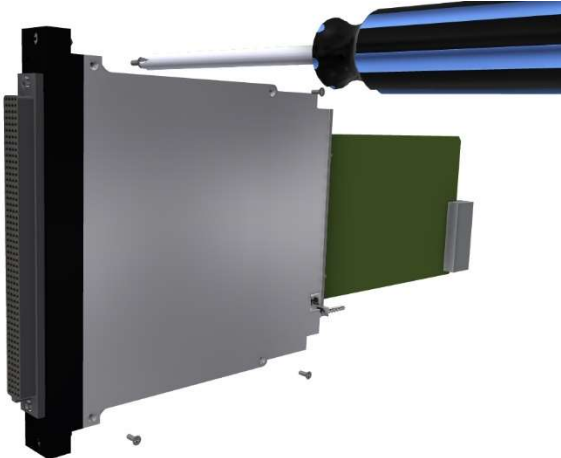
Figure 17 Attach right cover plate
