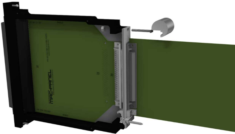
Figure 13 Use alignment tool to ensure that T bolt is correctly aligned.
