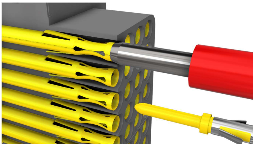
Figure 22 Probe inserted.
