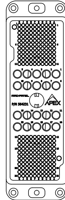
Mating Face View
