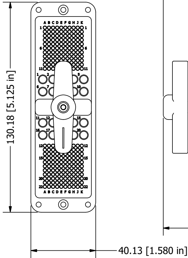
Wiring Face View
