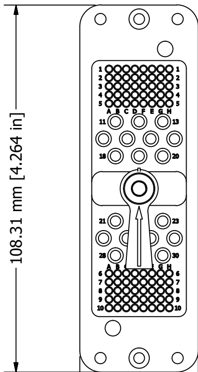
WIRING FACE VIEW
