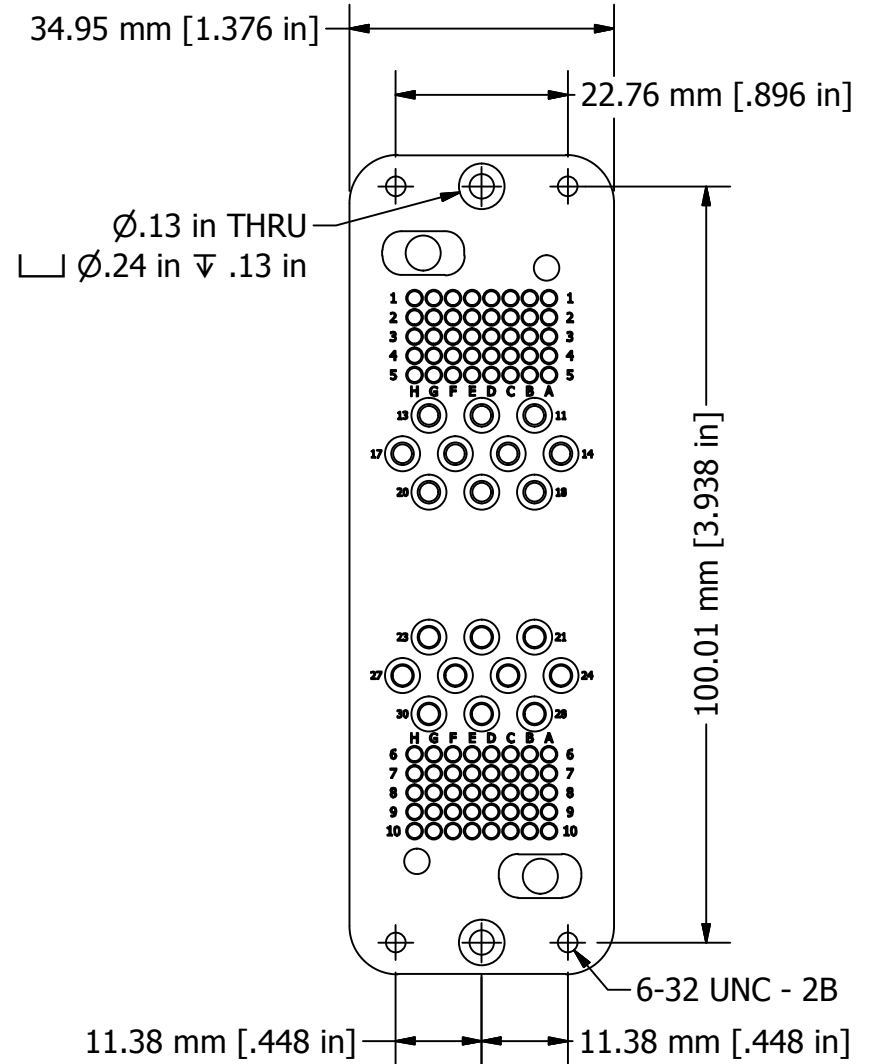
WIRING FACE VIEW
