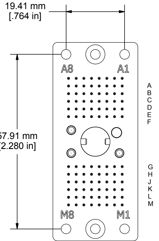
Socket Rear View
