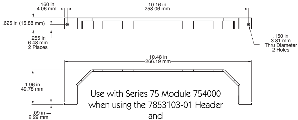
Strain Relief Bracket Part # 754000SR-04
