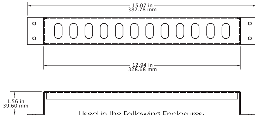
Strain Relief Bracket Part # 11705-03
