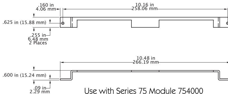
Strain Relief Bracket Part # 754000SR
